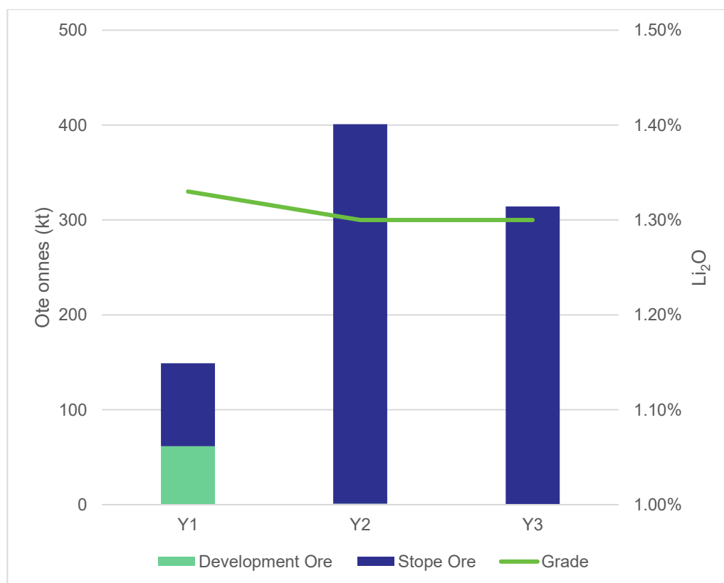
Figure 8 Grants Underground Production Schedule
